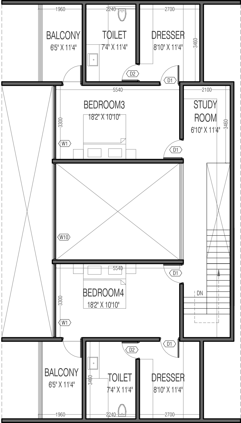
4BHK TYPE1- upper level
