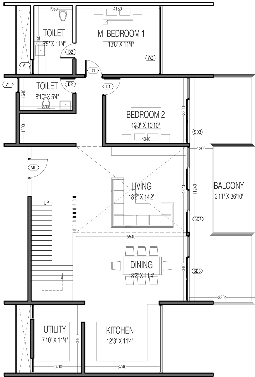
4BHK TYPE2 - lower level
