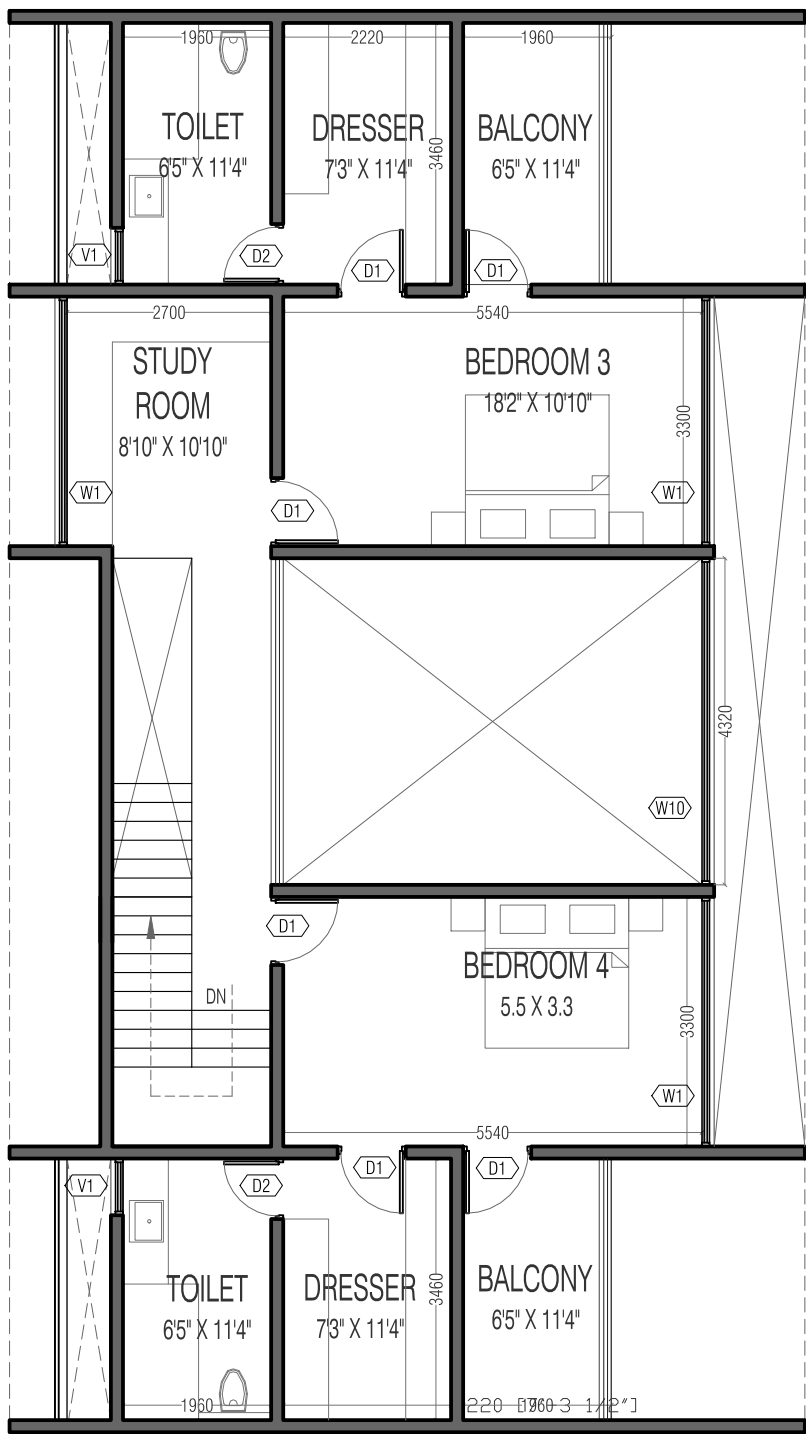
4BHK TYPE2 - upper level
