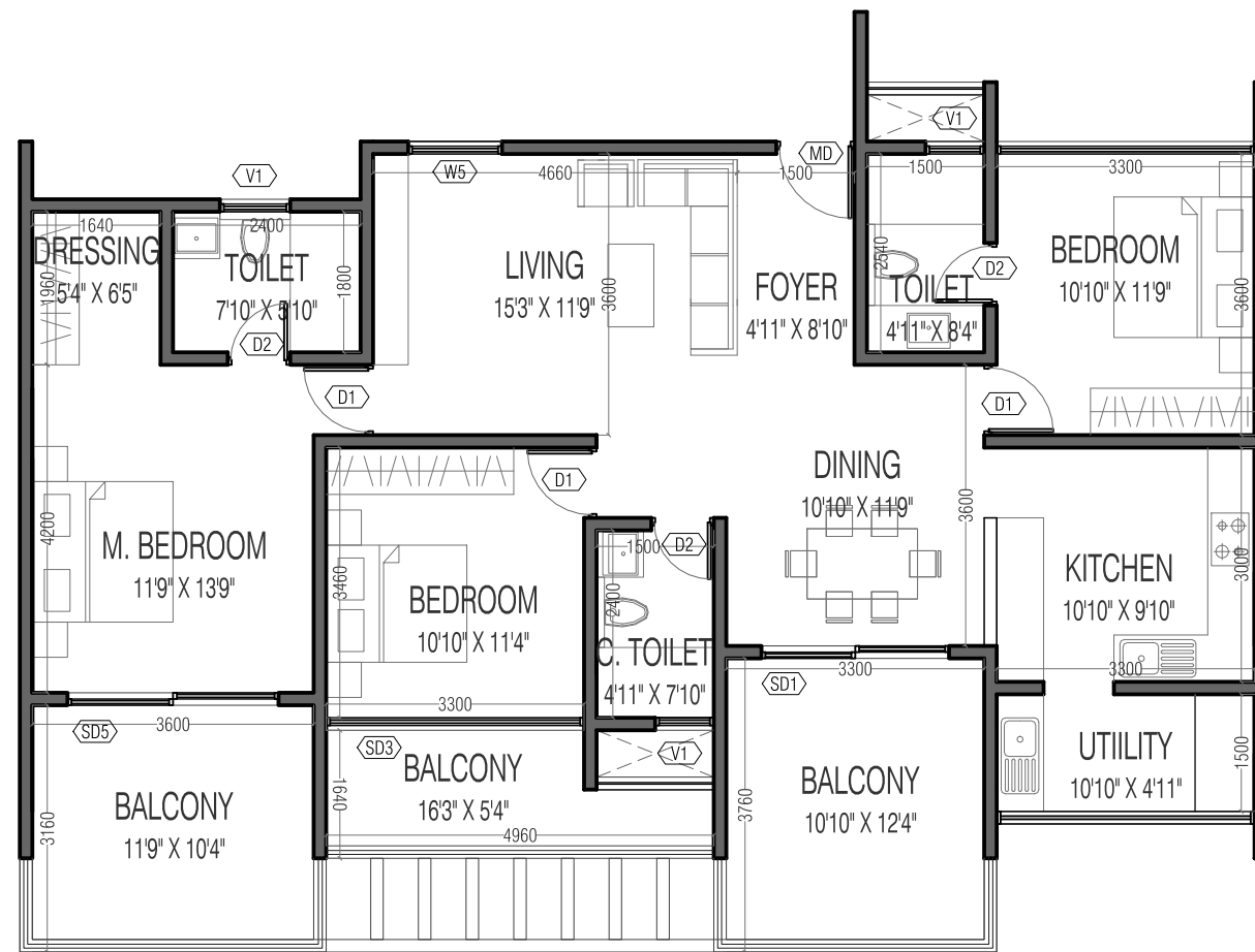
3BHK TYPE 2D
